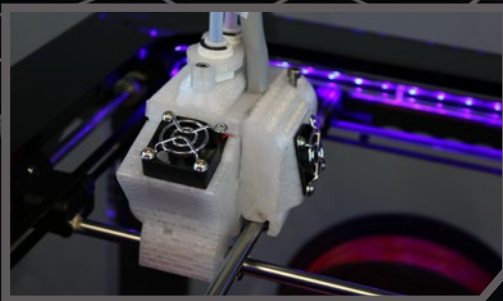
New and improved JR2x hotend features second cooling fan and easy calibration.
